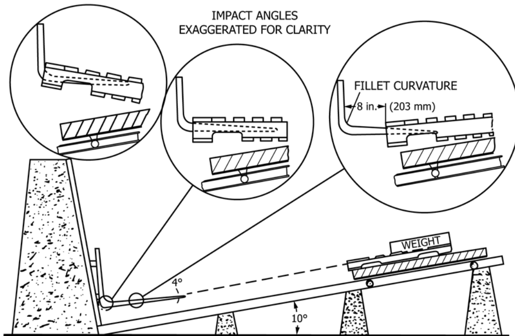
FIG. 9 Test Setup for Determination of Incline-Impact Resistance of Leading-Edge Deckboard of Pallet
