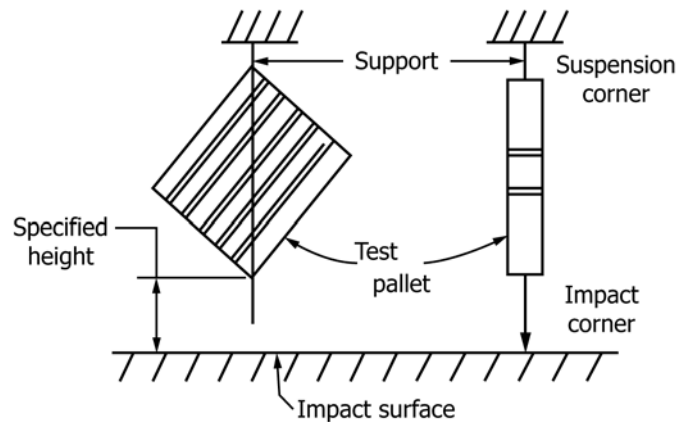
FIG. 6 Corner Drop of Vertically Suspended Pallet
