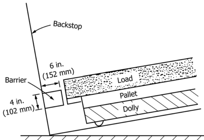
FIG. 10 Hazard Used for Impact Testing of Collapse Resistance
