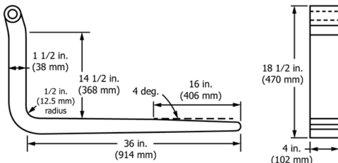
FIG. 8 Standard Fork Used for Leading-Edge Deck-Board-Separation Impact Test
