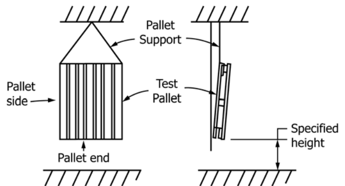
FIG. 7 End Drop of Vertically Suspended Pallet
