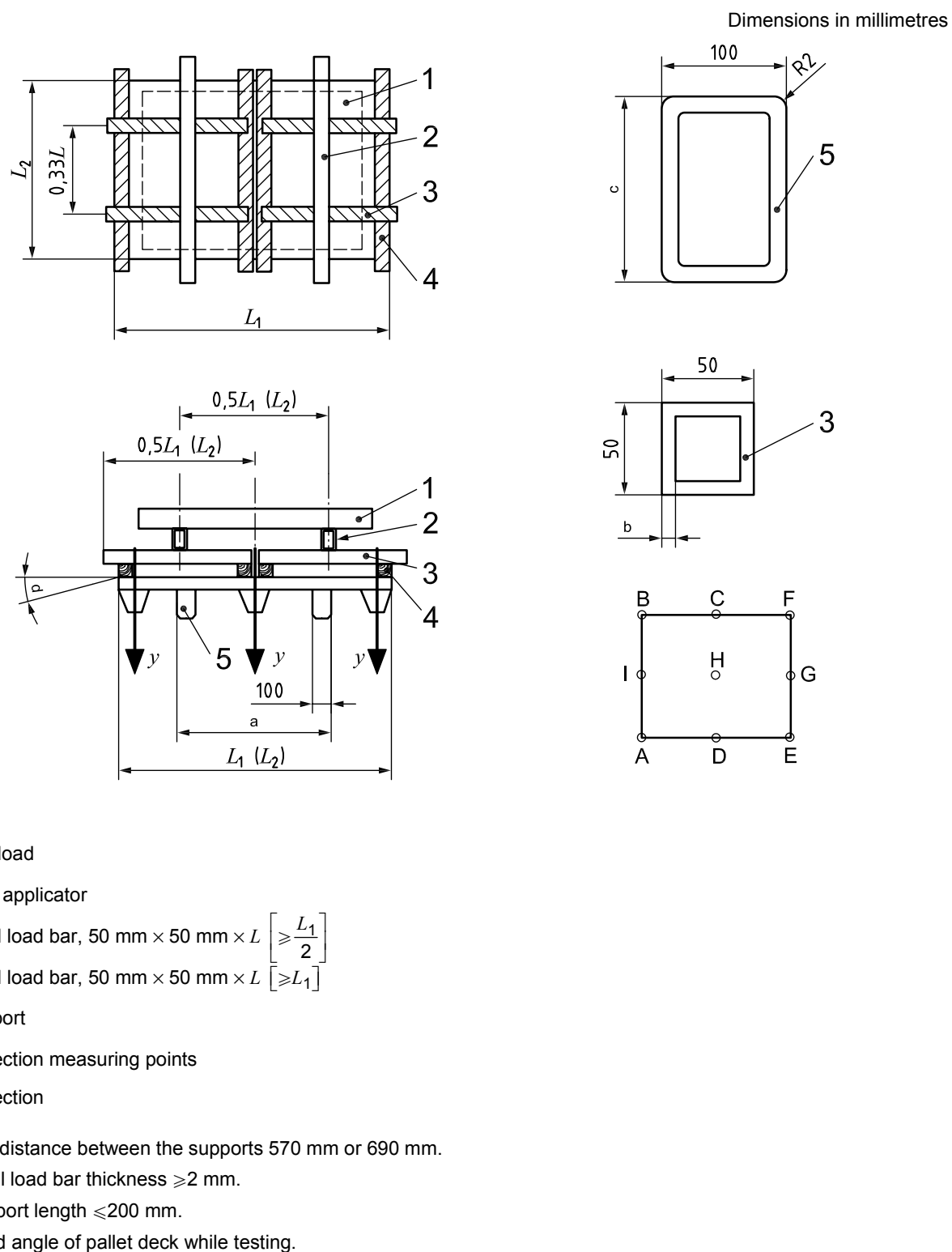
Figure 2 — Forklifting test
